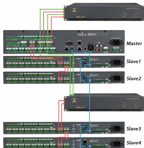
DIVA8MG2 Master unit and DIVA8SG2 Slave unit with 4 amplifier channels
