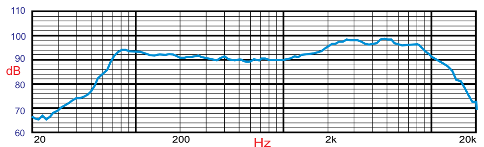
Frequency response
