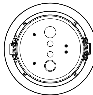
Rear view (unit: mm)
