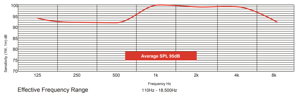
Frequency response
